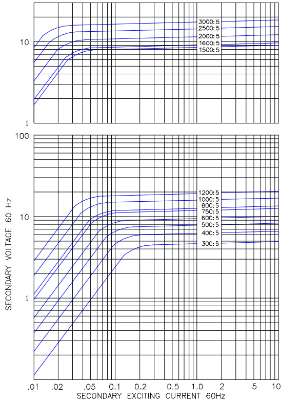
EXCITATION CURVE
